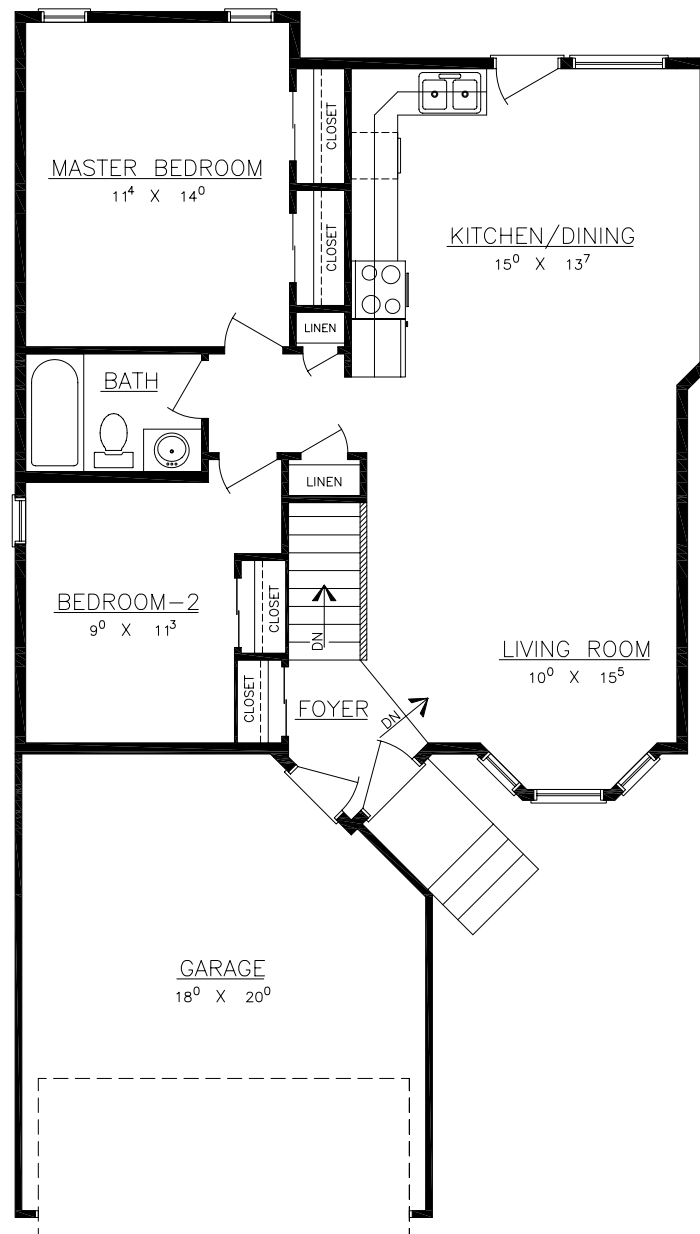
FLOOR PLAN
